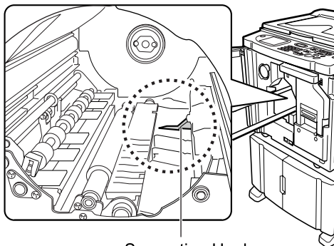
Separation Hook
